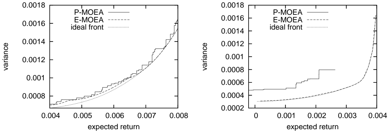
Figure 4: Typical fronts obtained on test problem P1 (left) and test problem P3 (right) with cardinality constraint.
