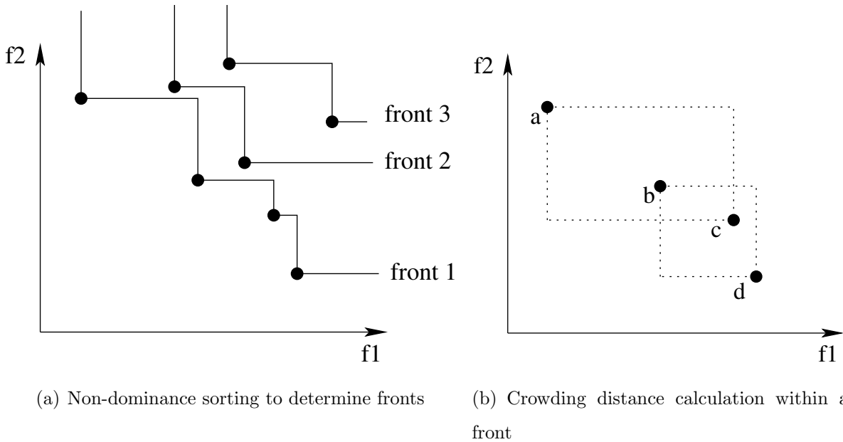
Figure 1: NSGA-II first ranks individuals according to non-dominance sorting (a) and within a front according to crowding distance (b).
