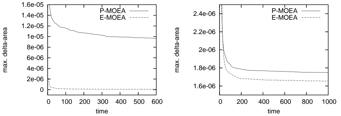
Figure 6: Convergence curves for P3 with cardinality constraint (left) and 5-10-40 constraint (right).
