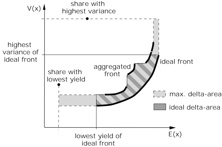
Figure 3: Ideal and maximum \Delta -area.
