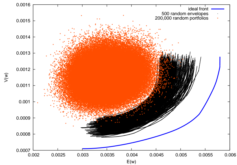
Figure 7: Randomly initialized populations of envelopes and portfolios for the 5-10-40 problem and the Hang Seng Dataset.
