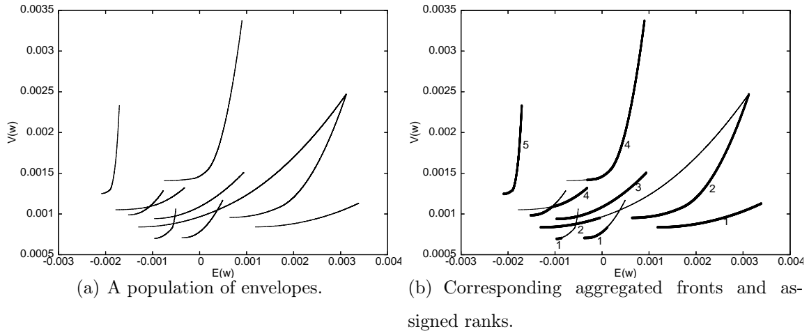
Figure 2: Ten randomly initialized envelopes and the five corresponding aggregated fronts for the max-card problem with k = 4 for the Nikkei dataset.
