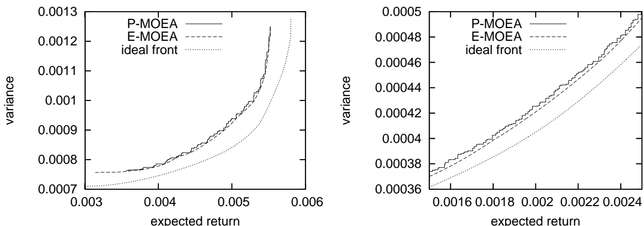
Figure 5: Typical fronts obtained on test problem P1 (left) and test problem P3 (right) with 5-10-40 constraint.
