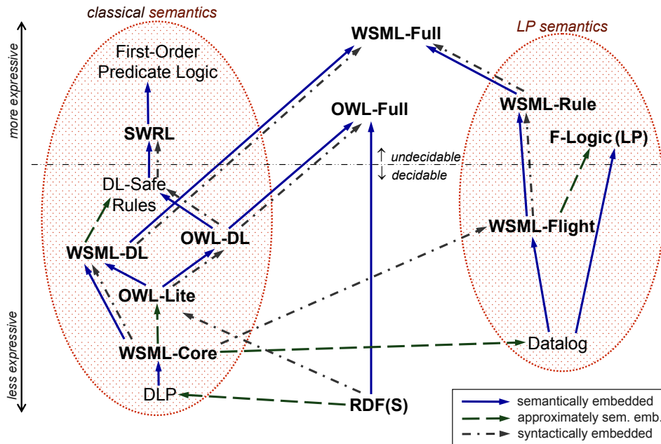
Fig. 3.4. An overview of Semantic Web languages
