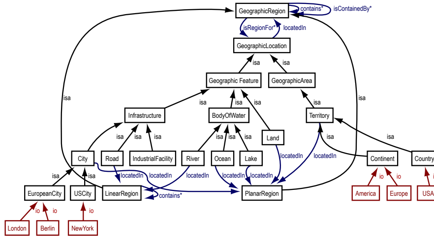
Fig. 3.2. A graphical visualisation for a geographic ontology
